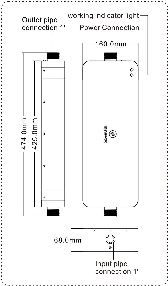
UVC-LED Whole House Water Sterilization System 50L/min
