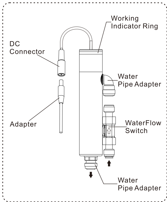
15L UVC-LED Water Sterilizer
